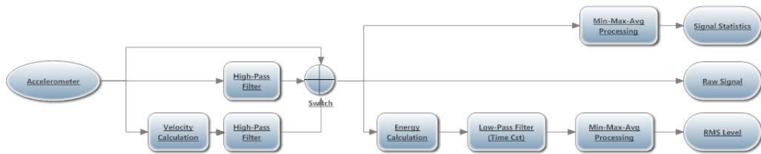
Figure 2 Signal Processing
