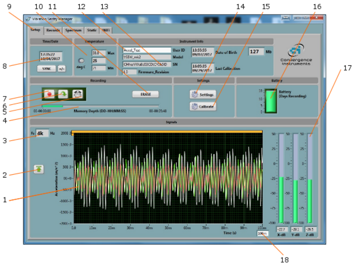
Figure 9 Setup Tab
