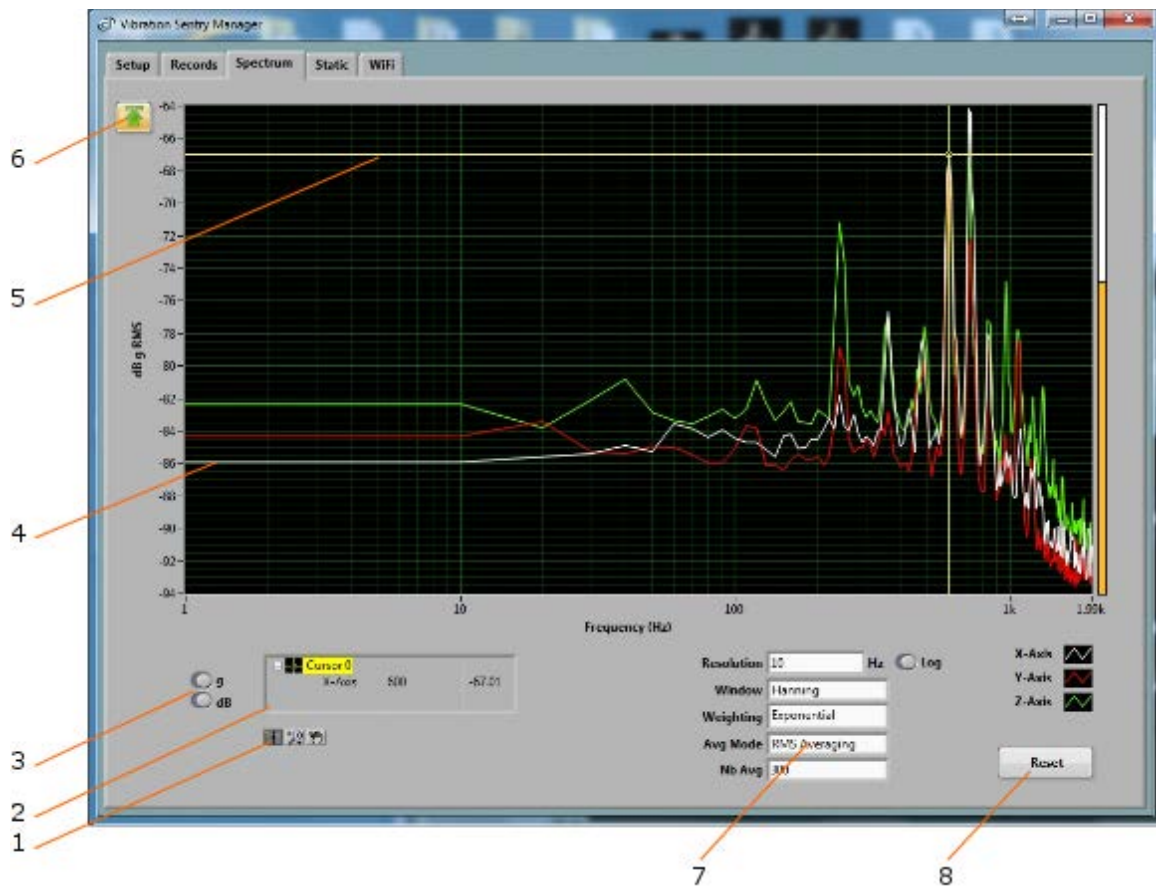
Figure 11 Spectrum Tab
